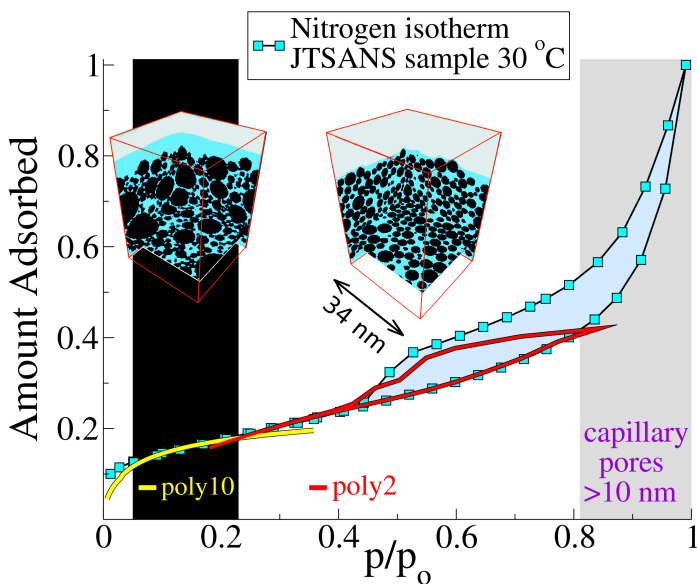
Comparison of experimental nitrogen sorption isotherm [exp. data from Dr. J. Thomas, Schlumberger Doll Research] with the theoretical results obtained using model C-S-H microstructures. “Poly2” and “Poly10” refer to low and high density C-S-H model microstructures, respectively.
